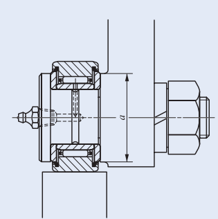
Fig. 1 Mating seating dimension "a"
