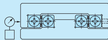
Fig. 24 Example of preload adjustment method
