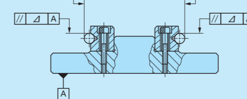
Fig. 28 Accuracy of way mounting
