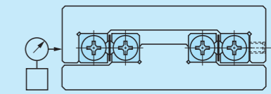
Fig. 31 Example of preload adjustment method
