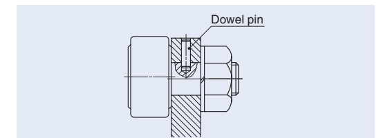
Fig. 6 Mounting example of Solid Eccentric Stud Type Cam Follower
