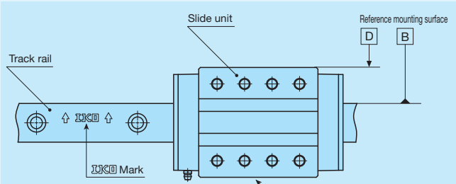
Fig. 4 Reference mounting surface
