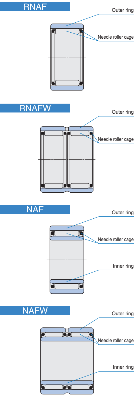
Structures of Needle Roller Bearings with Separable Cage
