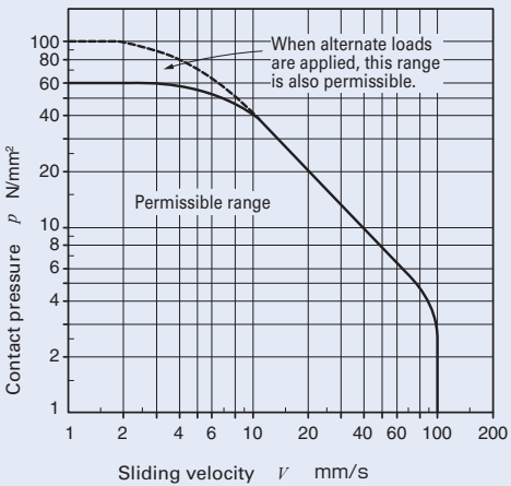
Fig.1 pV diagram of Steel-on-steel spherical bushings
