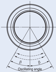
Fig.2 Oscillating angle
